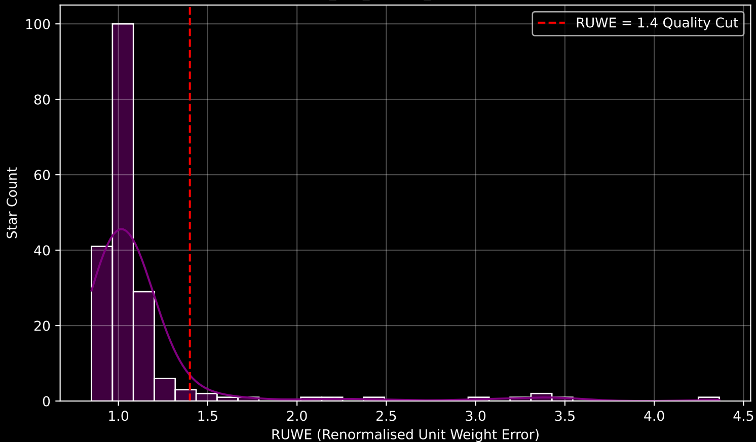
GAPOGEE DR17 Field [K2_C16_204+27_btx] RUWE Distribution (n= 192)
