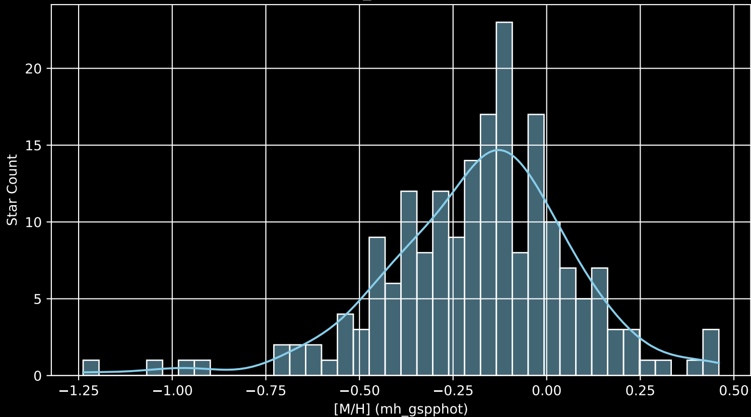
APOGEE DR17 Field: [K2_C16_204+27_btx [M/H] (mh_gspphot) (n= 194)
