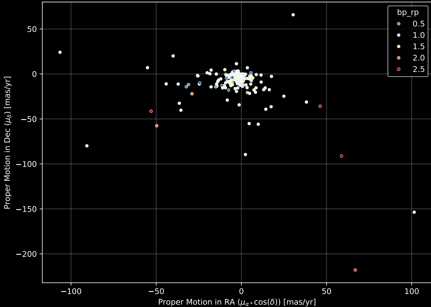
APOGEE DR17 Field: [K2_C16_204+27_btx] Proper Motion Diagram (n= 197)
