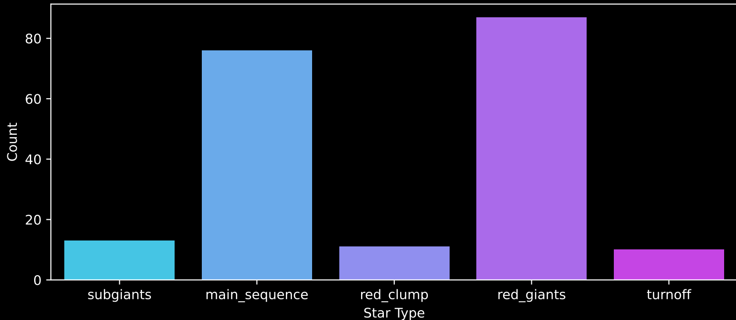
APOGEE DR17 Field: [K2_C16_204+27_btx] Count plot of Star Type
