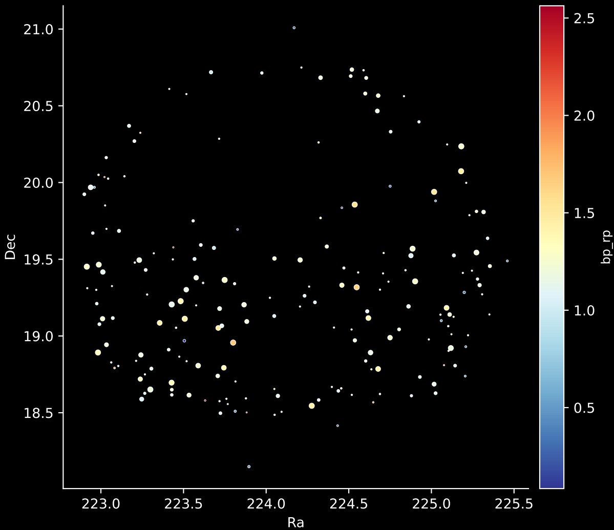
APOGEE DR17 Field: [K2_C16_204+27_btx] Stars: 197
