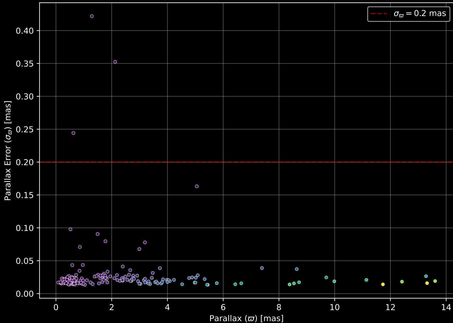
APOGEE DR17 Field: [K2_C16_204+27_btx] Parallax Quality (n= 197)
